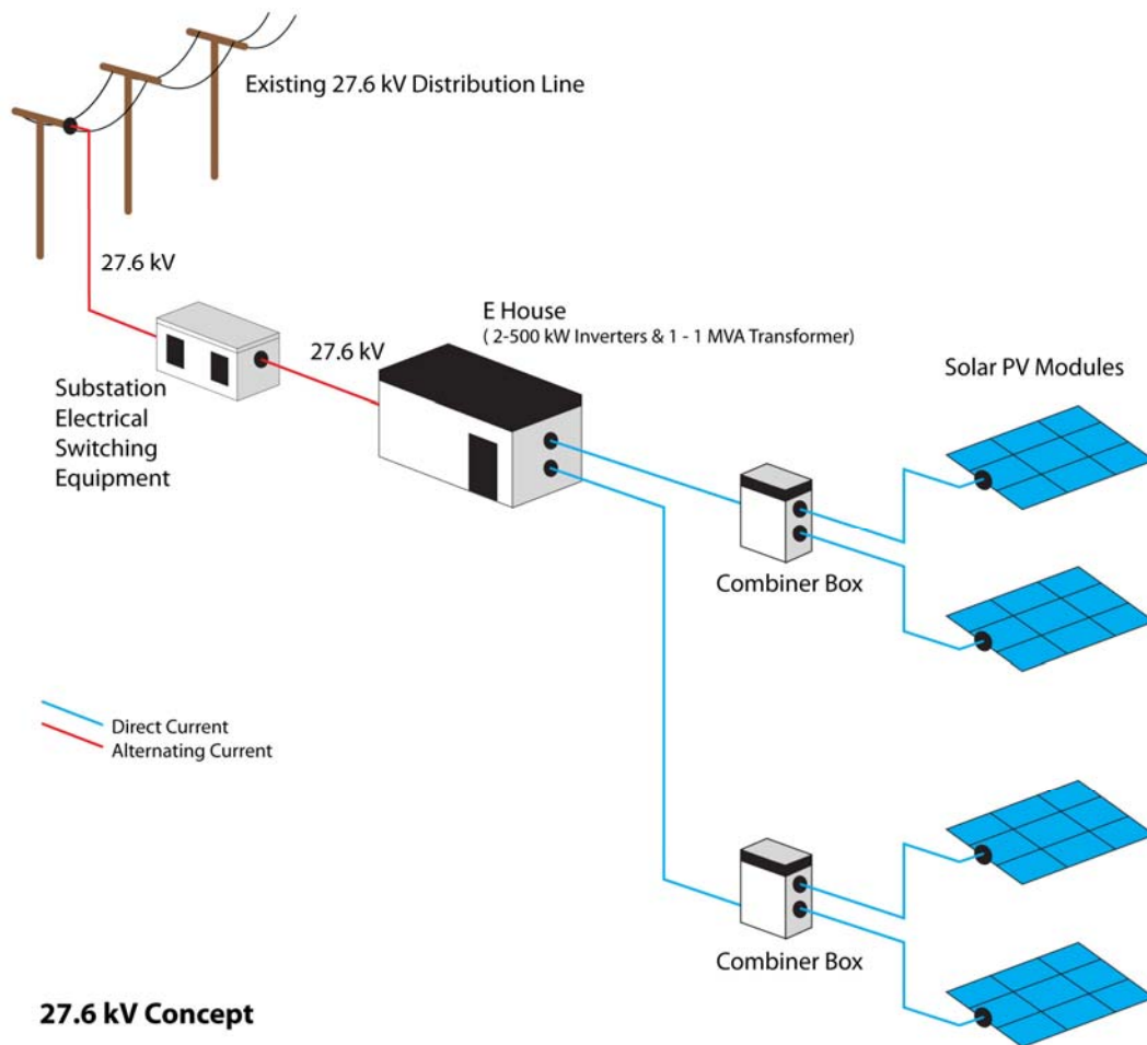
Figure 3.1 Generalized Schematic of Electrical Equipment Connectivity
